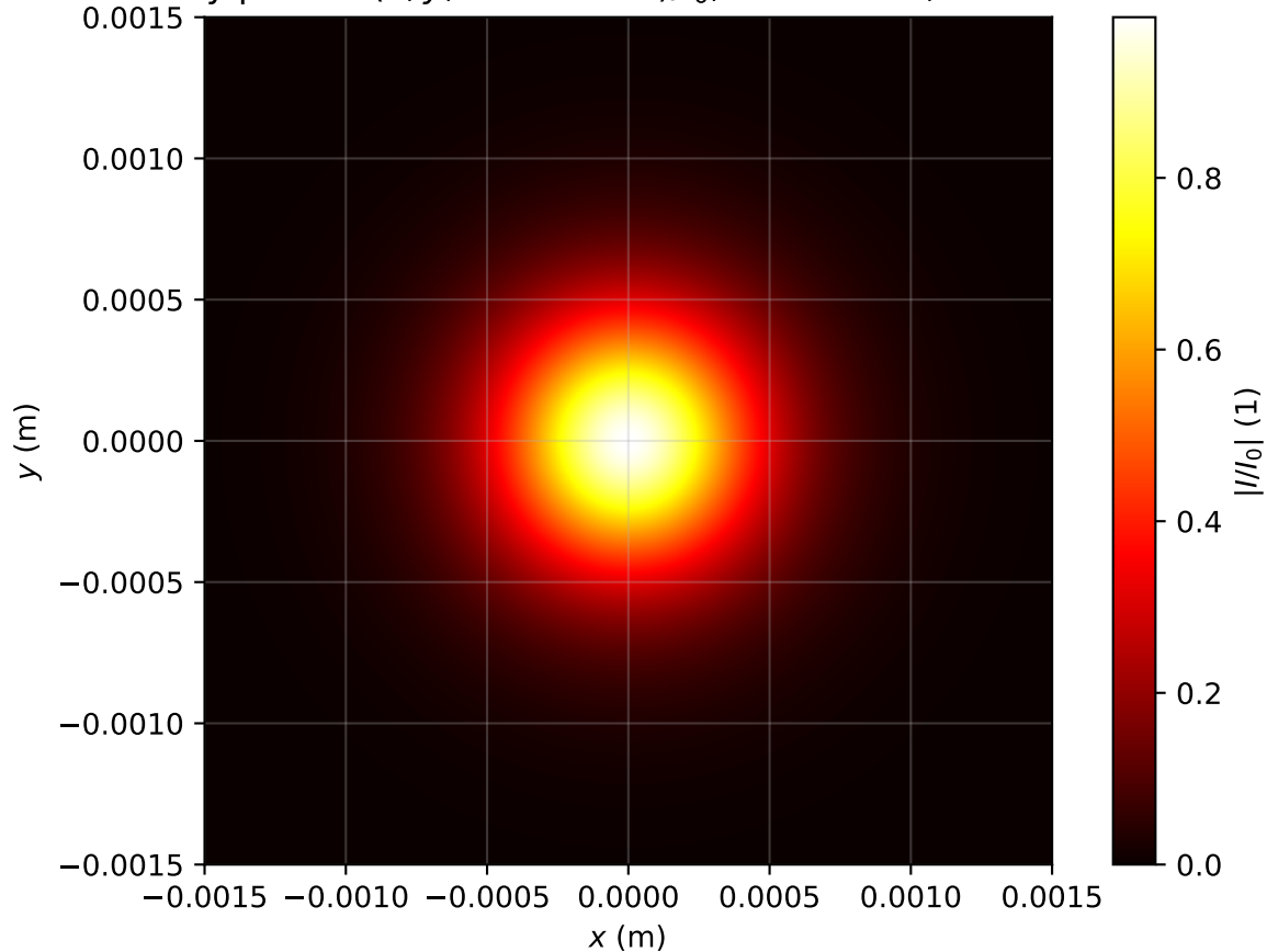
Intensity profile I(x, y, z = 1.831m)/I_0 , Pin=0.6Pcr, artificial time
